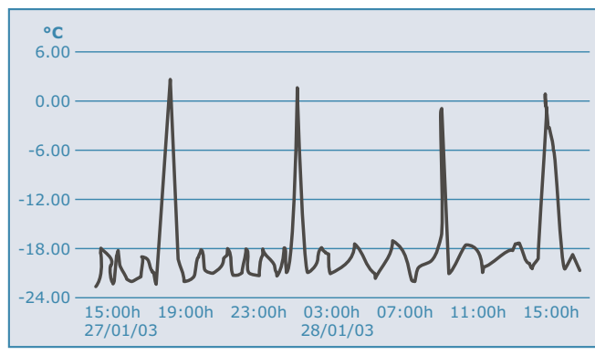
Fluctuation of temperature within 24 hours before the installation of the QKL:
